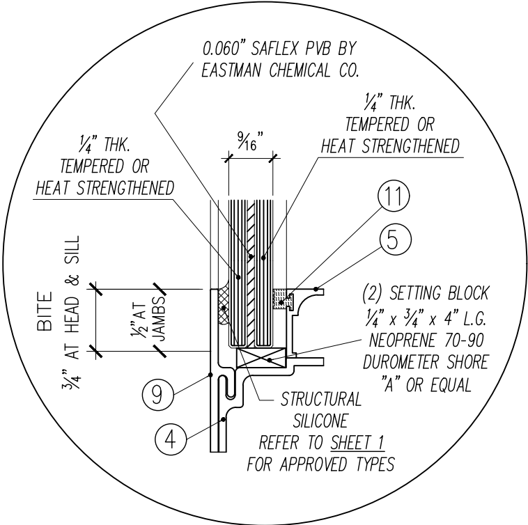
GLAZING DETAIL
